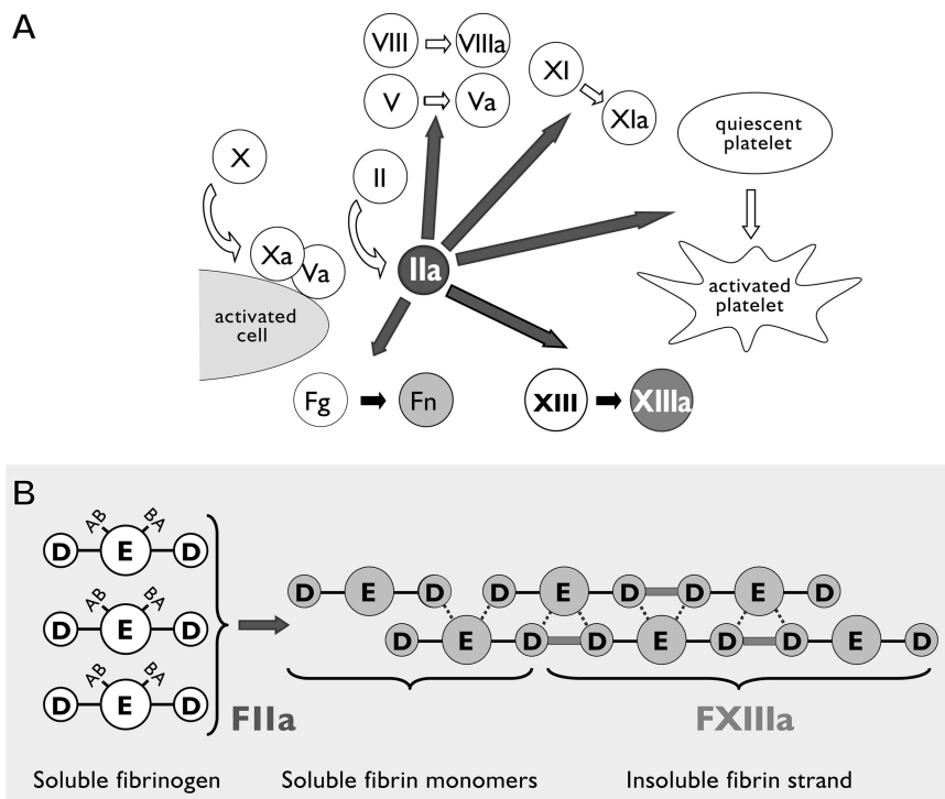
Fig. 1. Roles of thrombin in coagulation and roles of enzymatically active factor XIII (FXIIIa) in a simplified model of fibrin strand generation. (A) According to the cell-based model of coagulation, thrombin (IIa) is generated on the surface of activated cells ( left in A ) by FXa-mediated proteolytic cleavage from its precursor molecule, prothrombin. Thrombin ( dark gray ) is a key enzyme in coagulation and has multiple functions, including the activation of FXIII to generate FXIIIa. ( B ) Fibrinogen molecules comprise three domains: a central E domain flanked by two D domains. Fibrinogen is activated to fibrin monomers through the thrombin-mediated cleavage ( dark gray in B ) of the fibrinopeptides A and B from the E domain. Fibrinopeptide cleavage permits electrostatic interaction ( dotted lines ) of E domains with D domains of other fibrin molecules resulting in the formation of a still soluble fibrin strand. It is only after FXIIIa ( light gray ) has cross-linked fibrin monomers by covalently linking D domains of adjacent fibrin monomers ( bold light gray lines ) that the strands or protofibrils become “stabilized” or insoluble. Bottom graph ( B ) modified, with permission of Elsevier, from Furie B, Furie BC: Molecular basis of blood coagulation, Hematology: Basic Principles and Practice, 4th edition. Edited by Hoffman R. Philadelphia, Elsevier, 2005, pp 1946. Copyright © Elsevier 2005. 12
